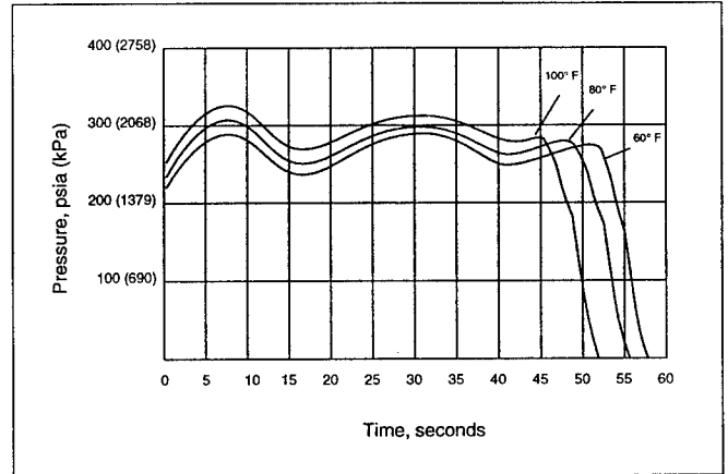
Figure 8: M57A1 Pressure vs. Time
