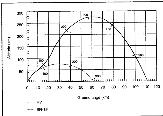
Figure 19: LC-32 Conventional Trajectory for HERA
