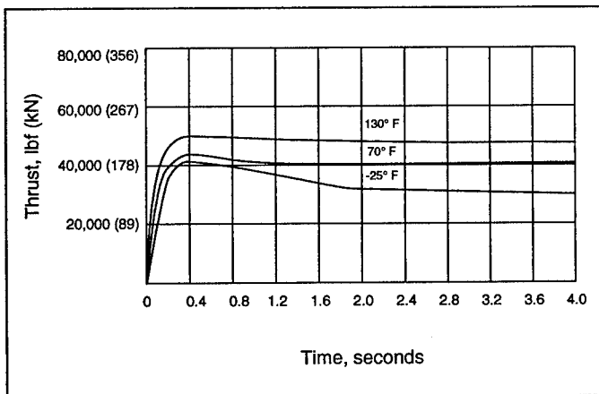
Figure 6: Sergeant XM100 Thrust vs. Time (Initial 4 Seconds)
