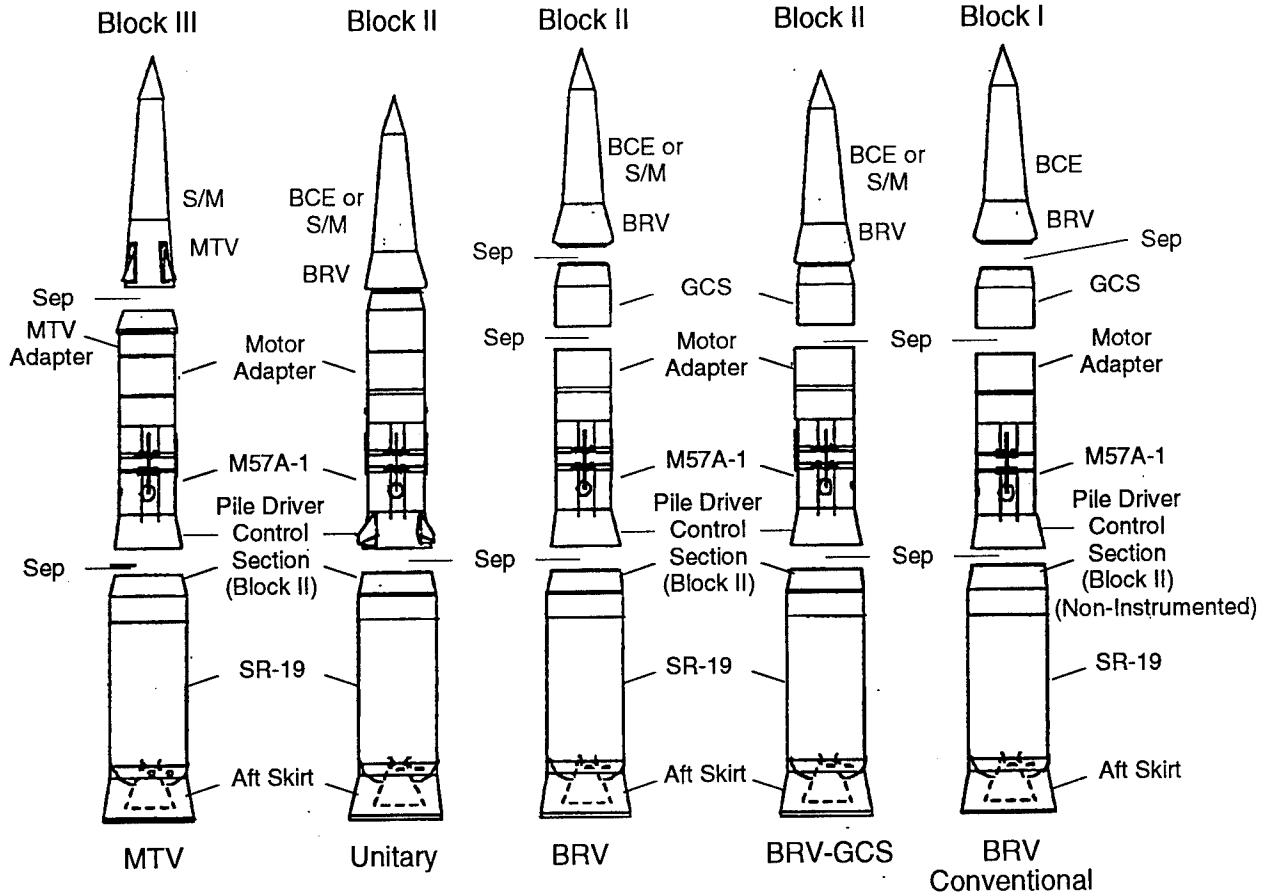
Figure17: HERA Target Configurations
