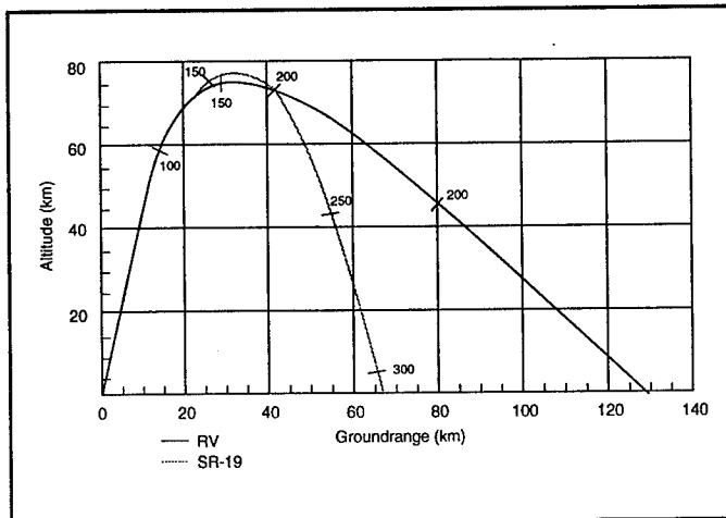
Figure 23: LC-32 Pile Driver Trajectory for HERA
