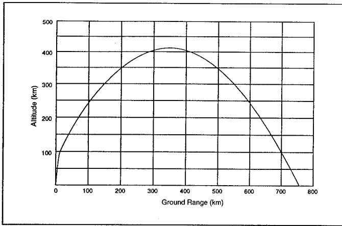
Figure 30: Strypi IX Altitude vs. Range
