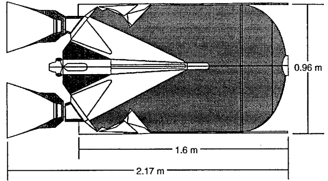
Figure 7: M57A1 Booster
