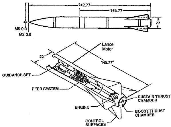
Figure 26: Lance Target System
