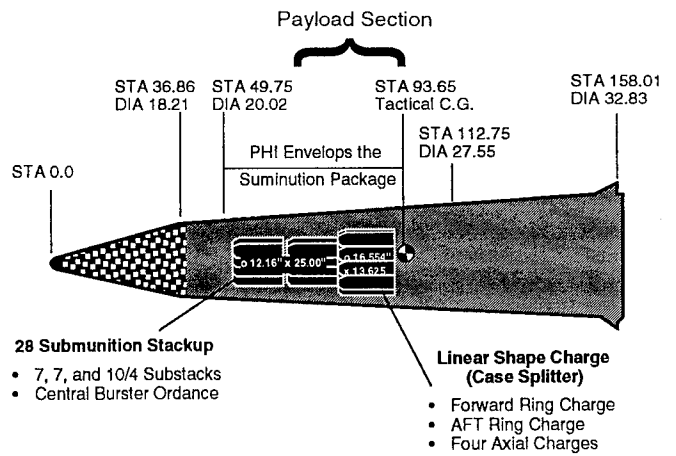
Figure 13: STORM MTTV
