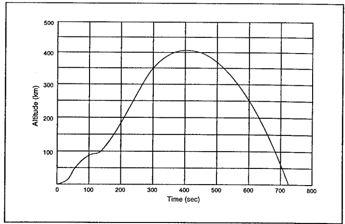
Figure 31: Strypi IX Altitude vs. Time
