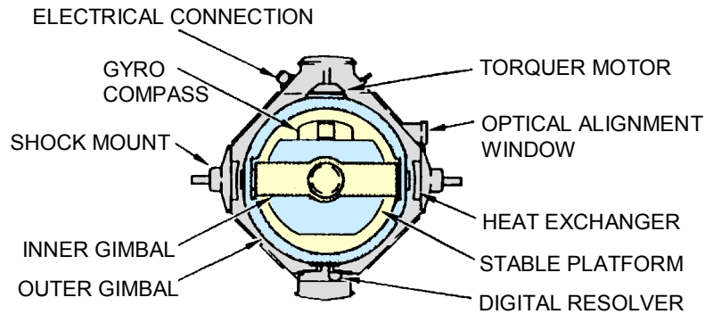
CROSS SECTION OF STABLE PLATFORM IN HOUSING
