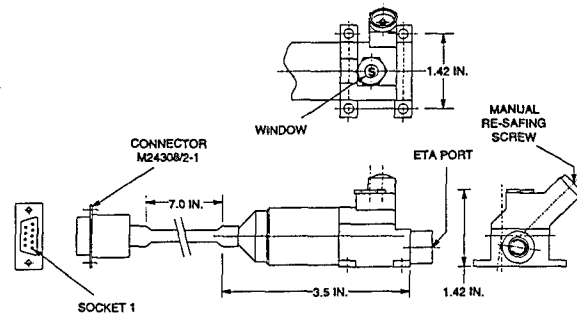
Figure 4. Safe-and-Arm Device
